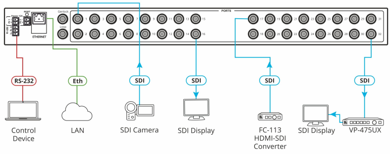
Figure 1. Rear Panel Connections
